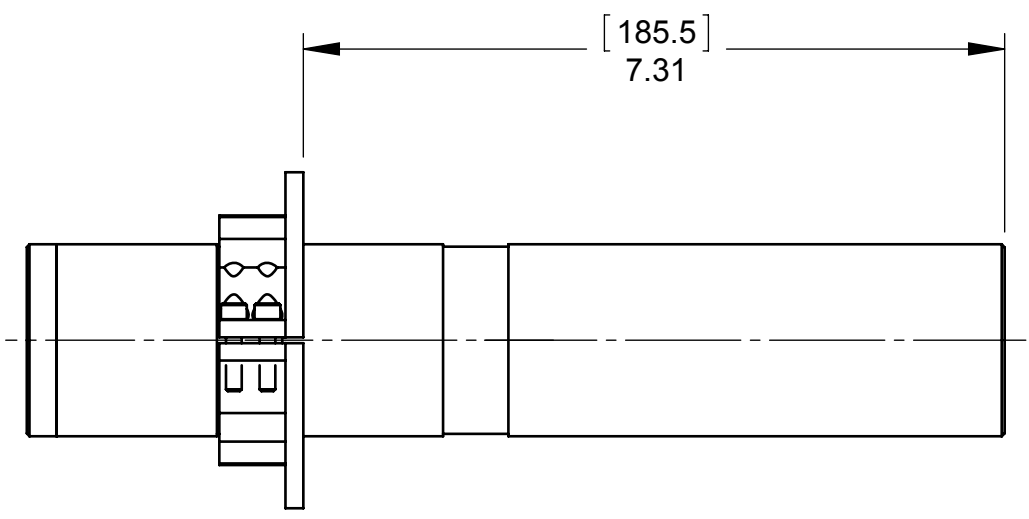
VIEW SHOWING FLANGE IN POSITION 2
