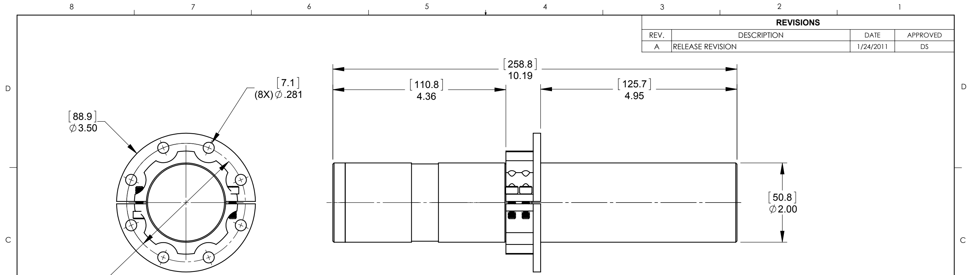
VIEW SHOWING FLANGE IN POSITION 1
