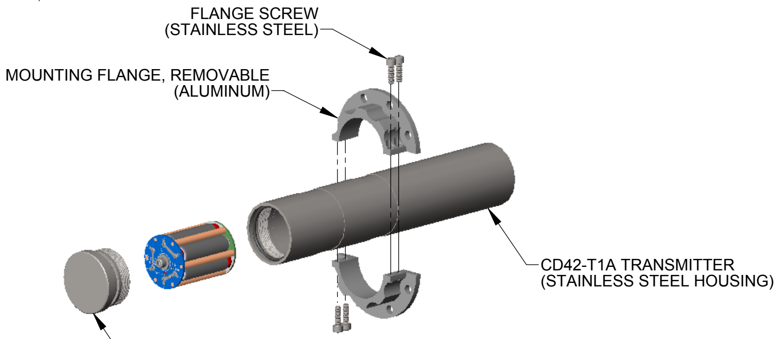
VIEW SHOWING FLANGE IN POSITION 1
